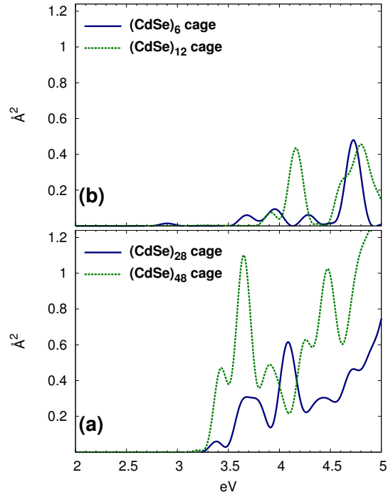
FIG. 4: (Color on line) Photoabsorption cross section of the empty cages. In panel (a) the absorption spectra of (\text{CdSe})_{48} (dotted line) and (\text{CdSe})_{28} (solid line); in panel (b) the absorption spectra of (\text{CdSe})_{12} (dotted line) and (\text{CdSe})_6 (solid line).
