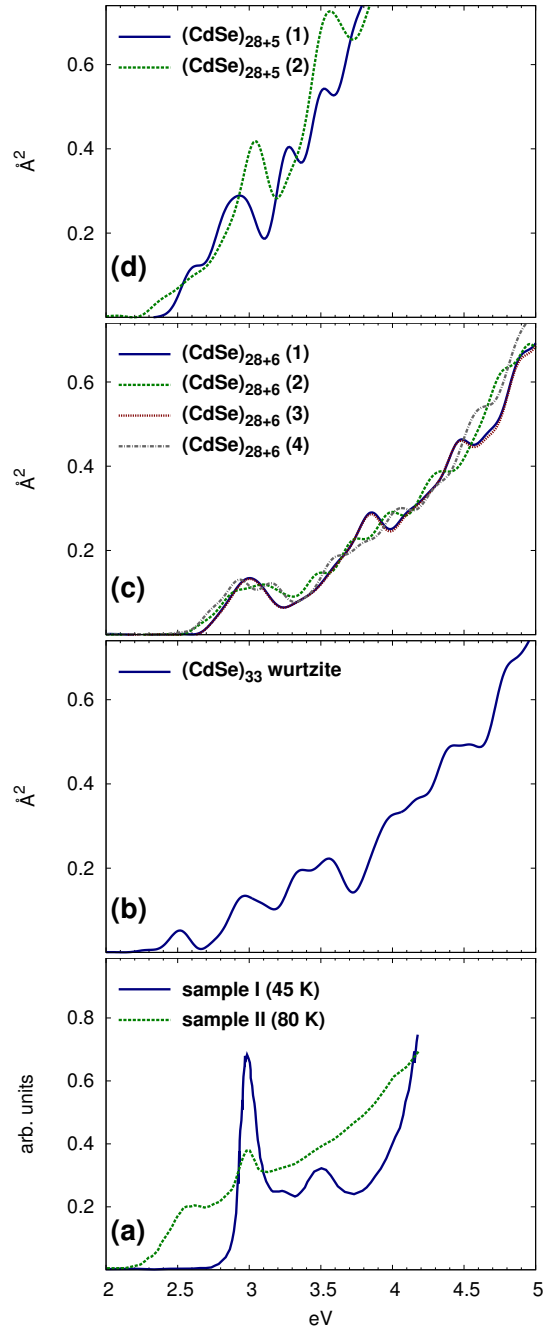
FIG. 6: (Color on line) Photoabsorption cross section of the isomers of (\text{CdSe})_{33,34} . The experimental data in arbitrary units (a) are compared with our calculated spectra (b), (c), and (d). The different curves in panels (c) and (d) correspond to distinct relaxed geometries obtained starting from different filled cages.
