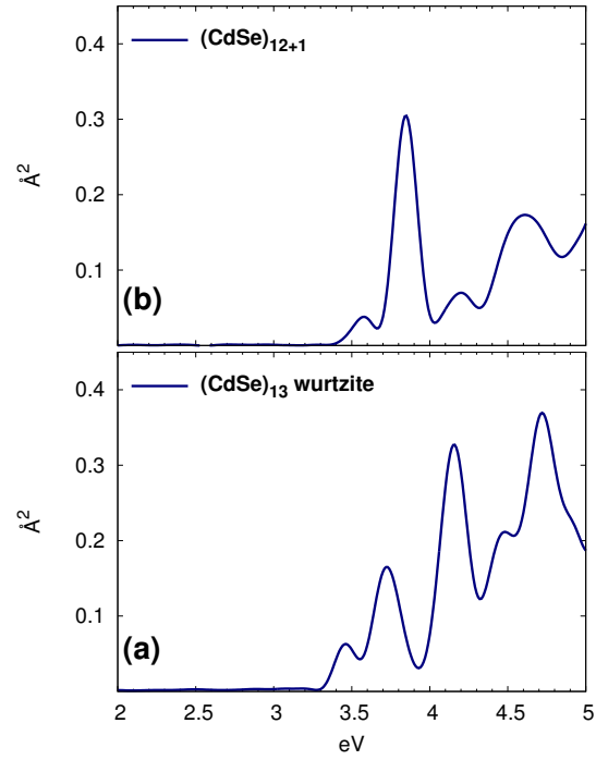
FIG. 5: (Color online) Photoabsorption cross section of the isomers of (\text{CdSe})_{13} . In panel (a) the absorption spectrum of the wurtzite structure; in panel (b) the absorption spectrum of the filled cage.
